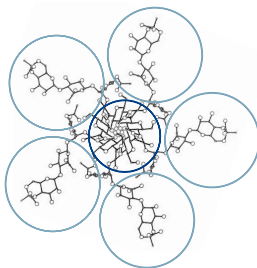
Top view of a xanthan gum molecule
